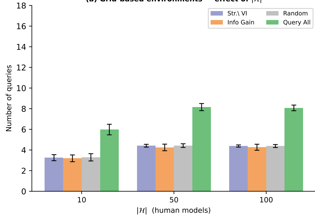
(a) Grid-based environments — effect of |\mathcal{H}|
