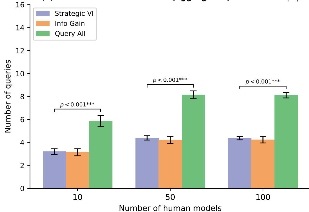
(a) Grid-based environments (aggregated) — effect of |\mathcal{H}|
