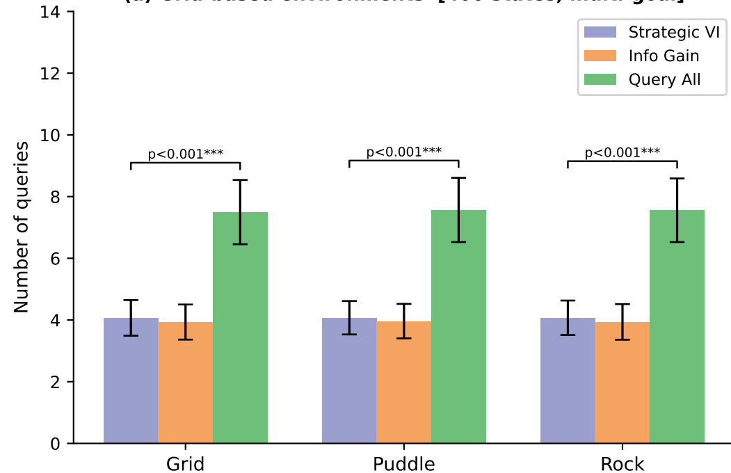
(a) Grid-based environments [400 states, multi-goal]
