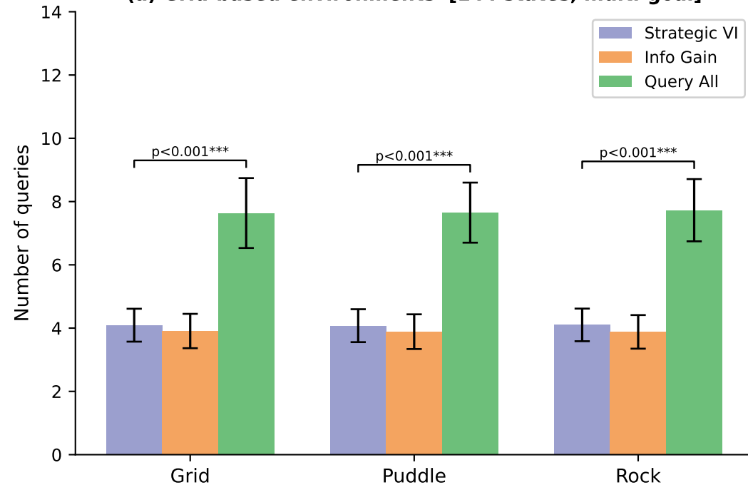
(a) Grid-based environments [144 states, multi-goal]
