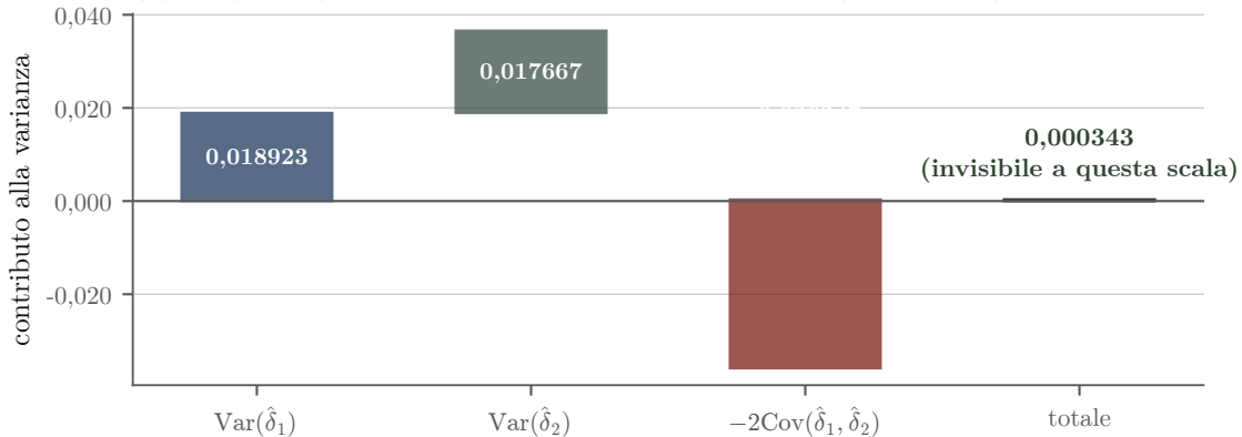
(a) \text{Var}(\hat{\delta}_1 - \hat{\delta}_2) : la covarianza cancella quasi tutto ( \rho = 0,9912 )
