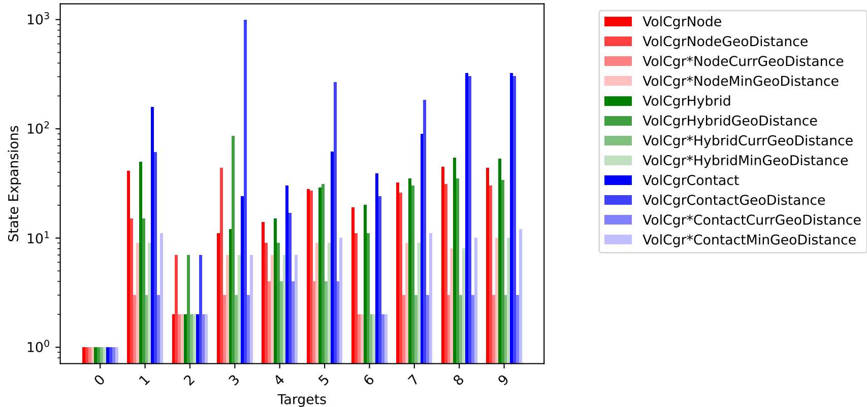
Comparison of the Number of State Expansions of VolCgr and VolCgr* for different Parenting Classes
