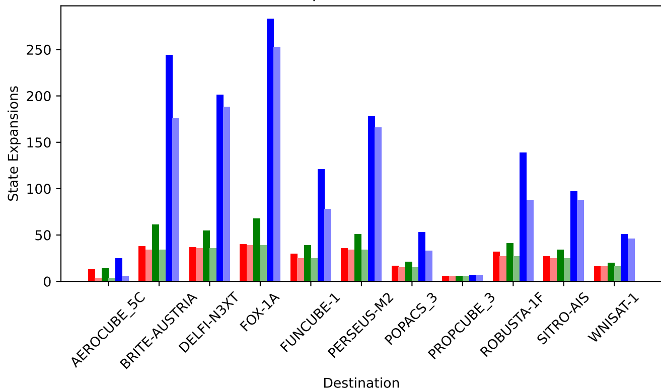
Number of State Expansions of VolCGR vs. VolCGR*
