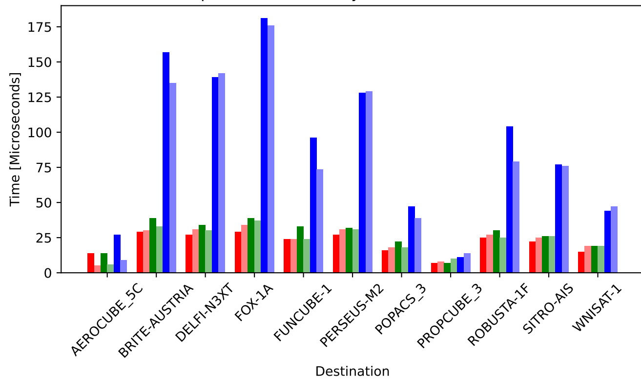
Computational Efficiency of VolCGR vs. VolCGR*
