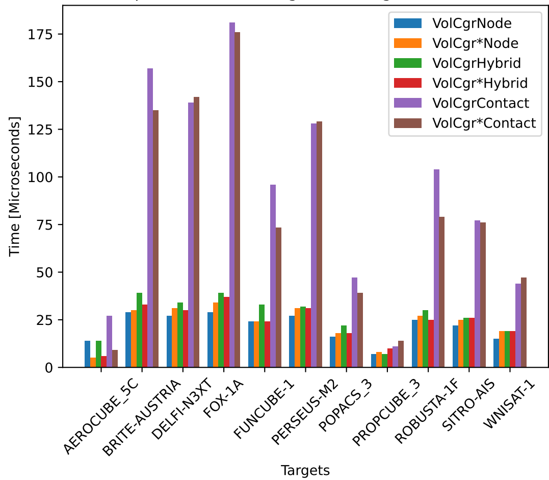
Comparison of the Required Time of VolCgr and VolCgr* for different Parenting Classes
