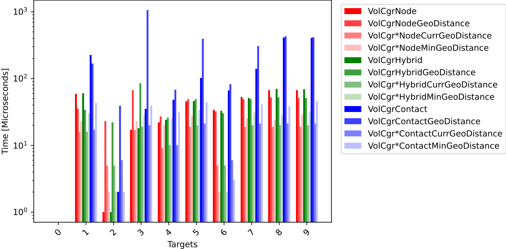
Comparison of the Required Time of VolCgr and VolCgr* for different Parenting Classes
