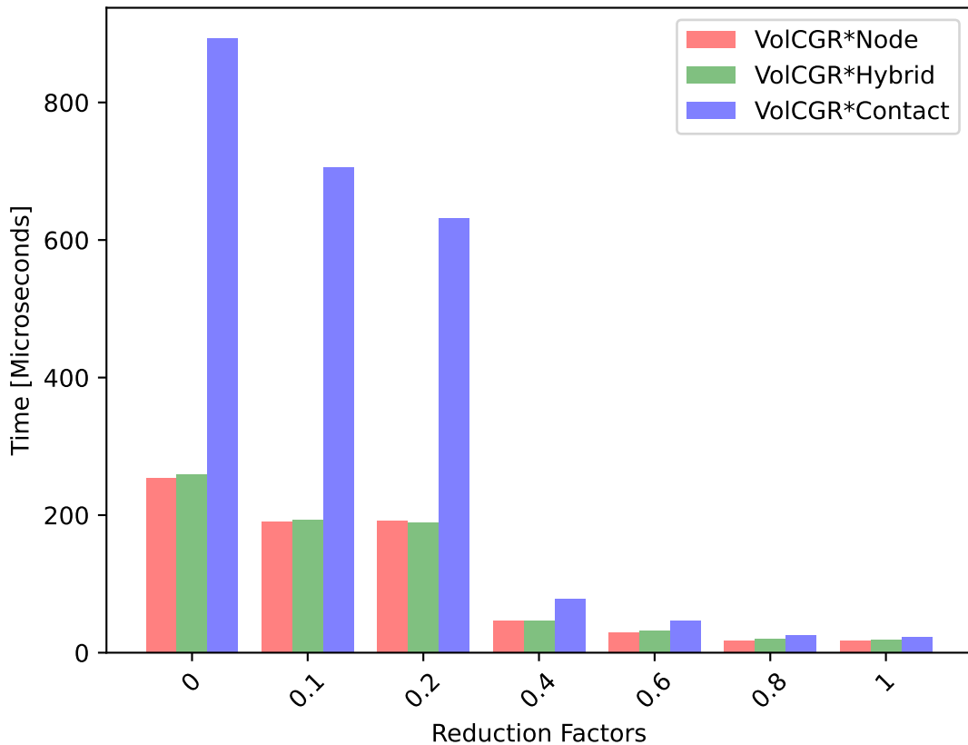
Computational Efficiency for different Reduction Factors of the heuristic
