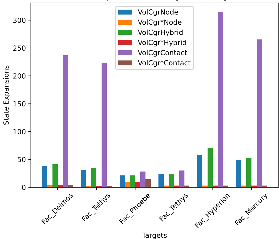
Comparison of the Number of State Expansions of VolCgr and VolCgr* for different Parenting Classes
