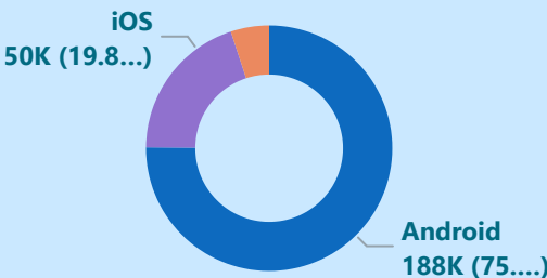
Device Type
