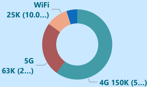
Network Type
