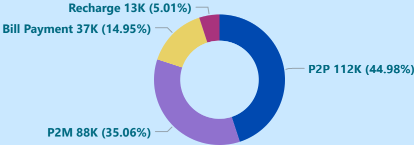
Transaction Type
