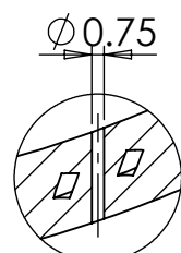
DETAIL C SCALE 2:1
