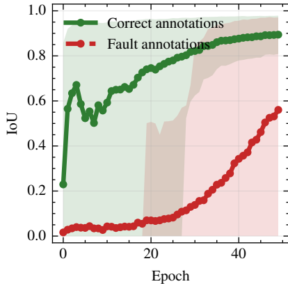
IoU over training
