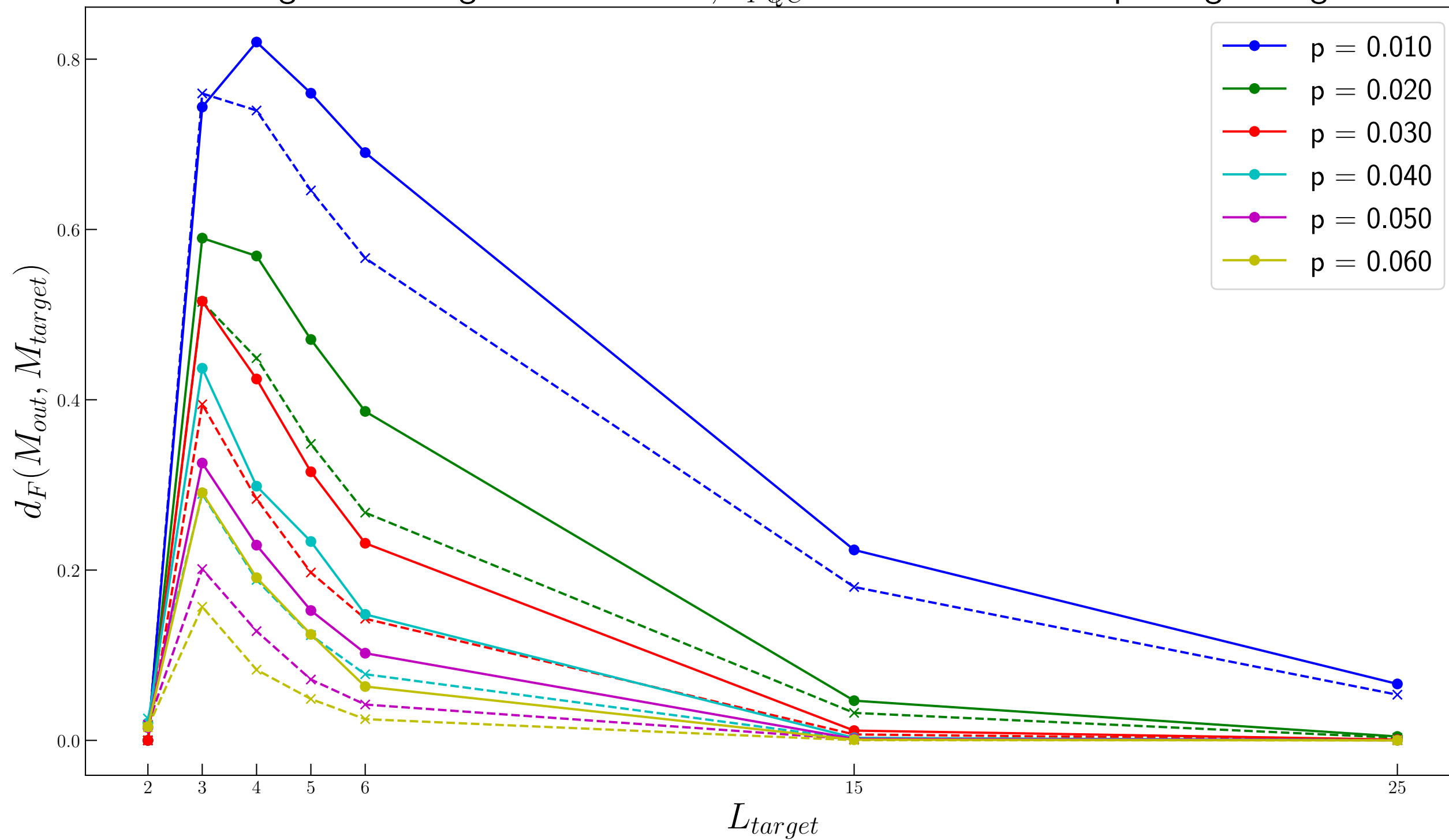
Learning and Testing Loss for N = 8, T_{PQC} = 2 with Various Dephasing Strengths
