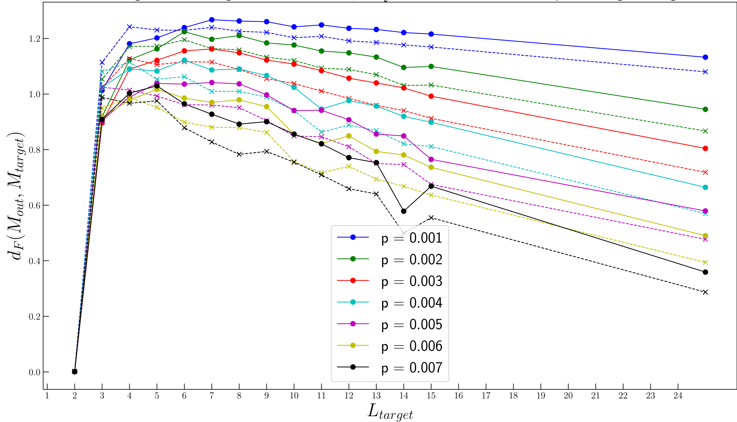
Learning and Testing Loss for N = 8, T_{PQC} = 2 with Various Depolarizing Strengths
