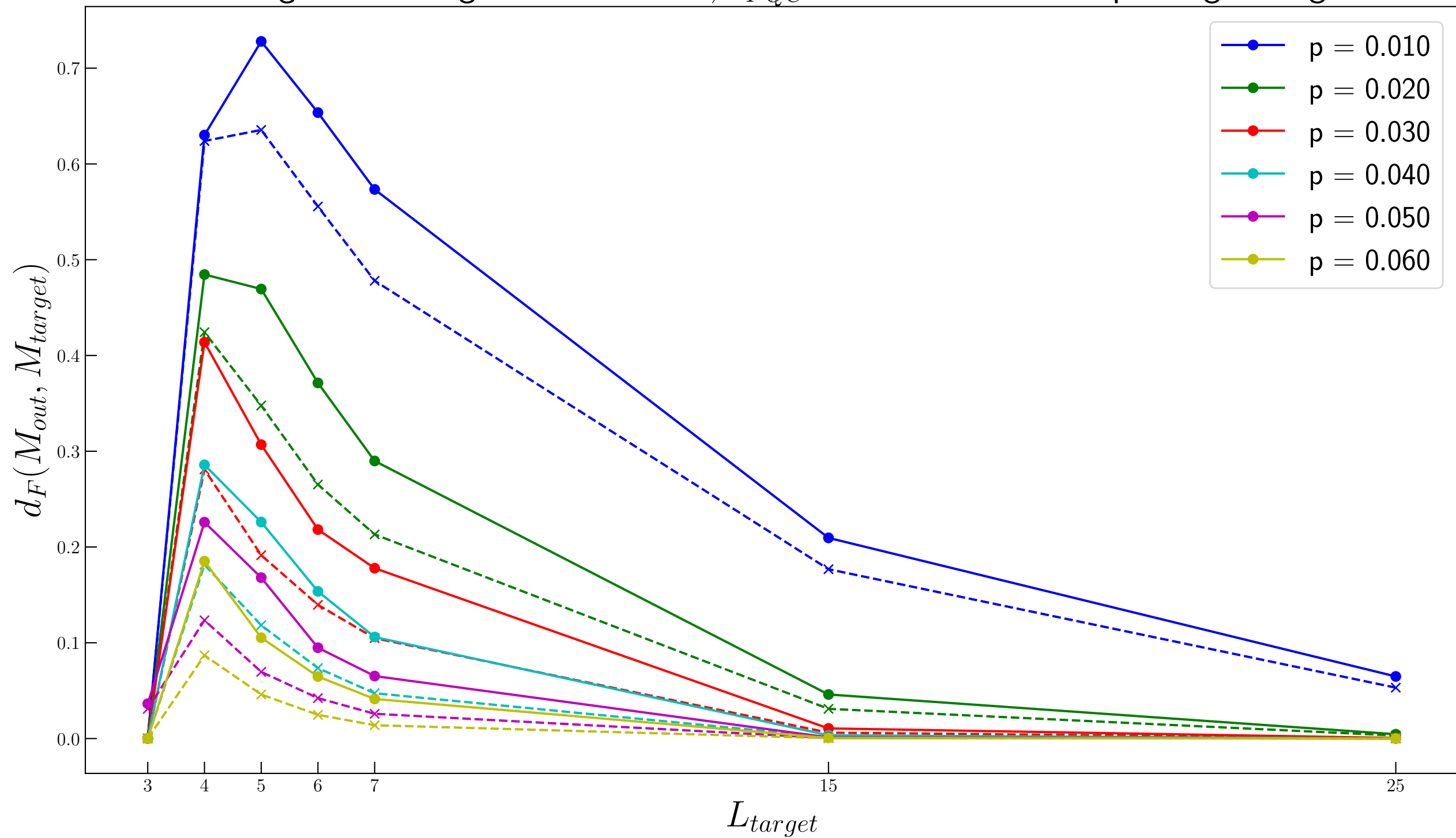
Learning and Testing Loss for N = 8, T_{PQC} = 3 with Various Dephasing Strengths
