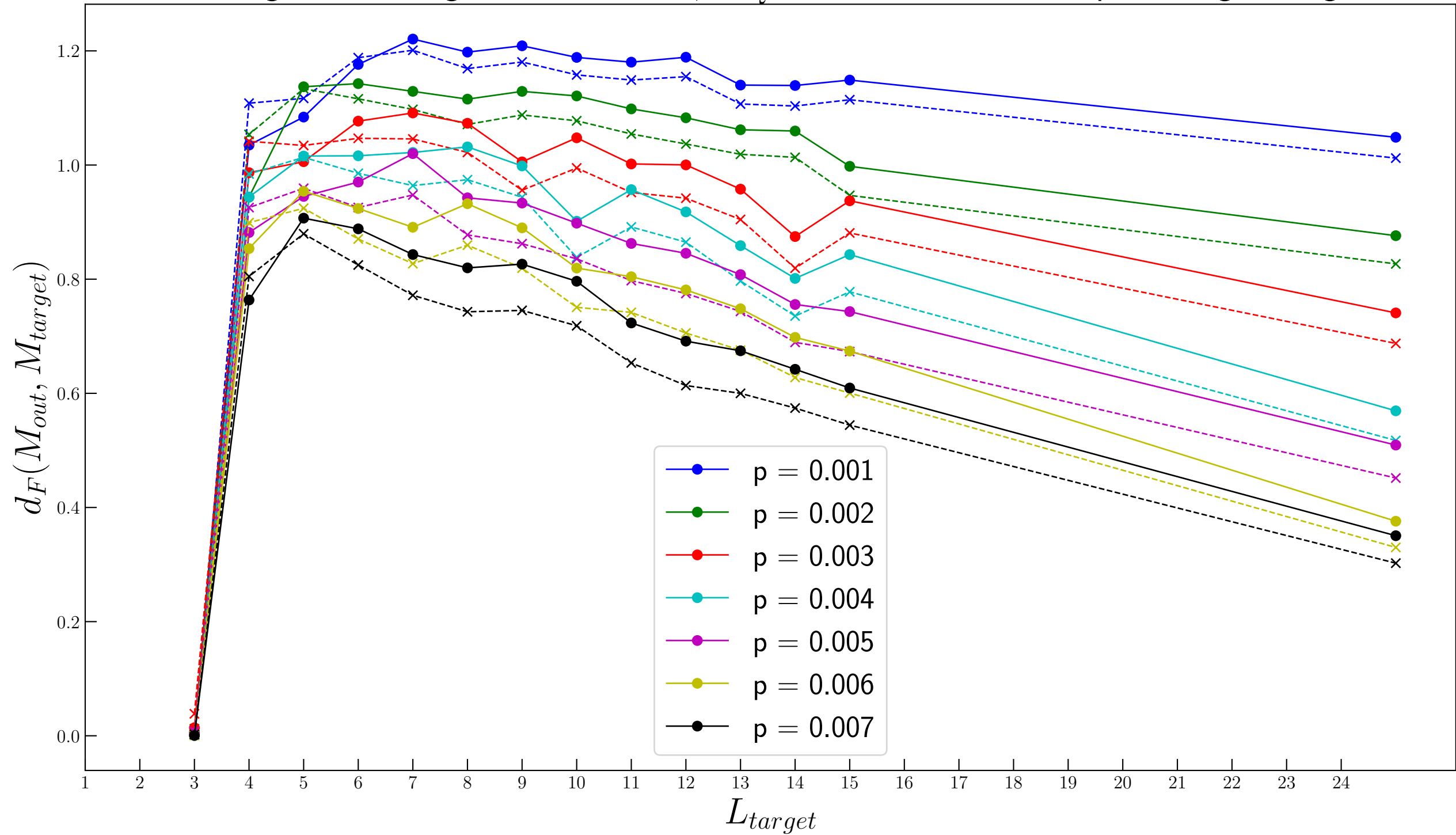
Learning and Testing Loss for N = 8, T_{PQC} = 3 with Various Depolarizing Strengths
