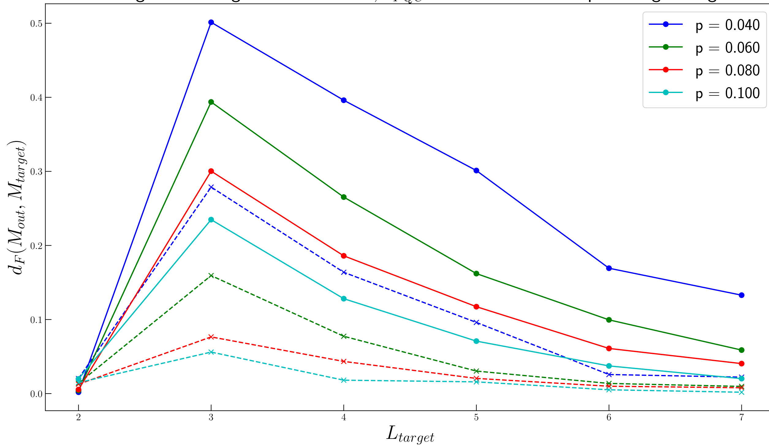
Learning and Testing Loss for N = 12, T_{PQC} = 2 with Various Depolarizing Strengths
