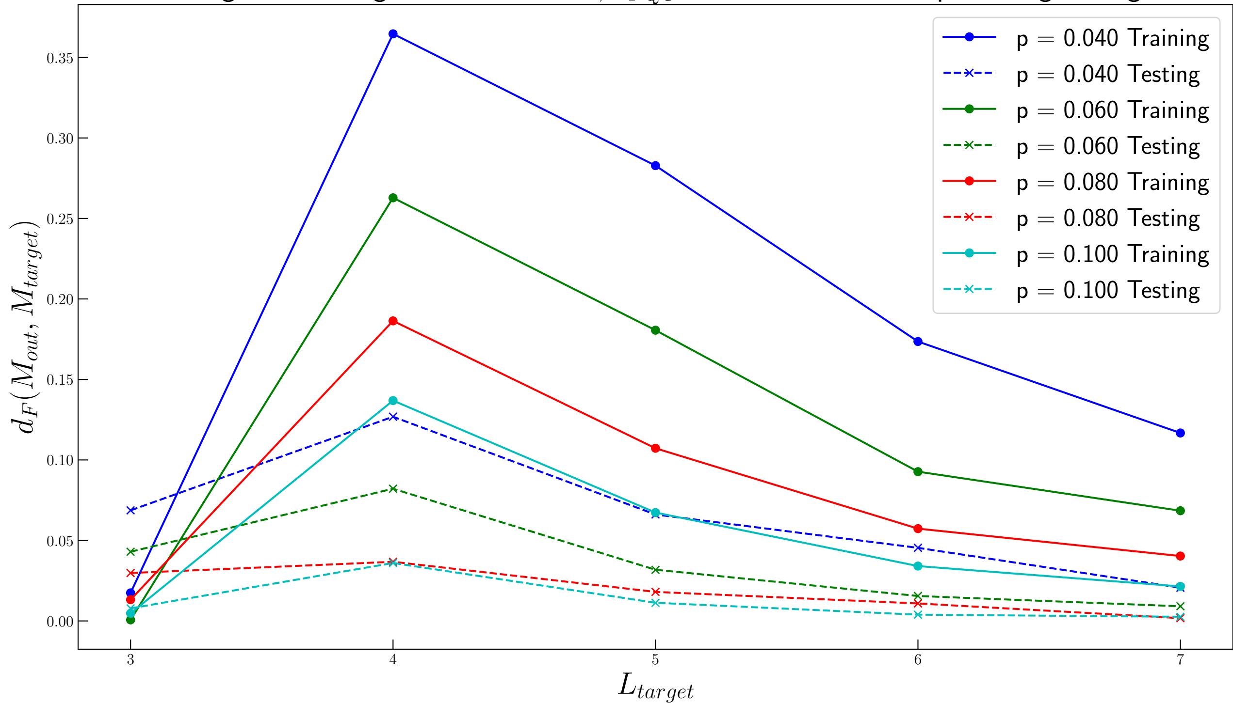
Learning and Testing Loss for N = 12, T_{PQC} = 3 with Various Depolarizing Strengths
