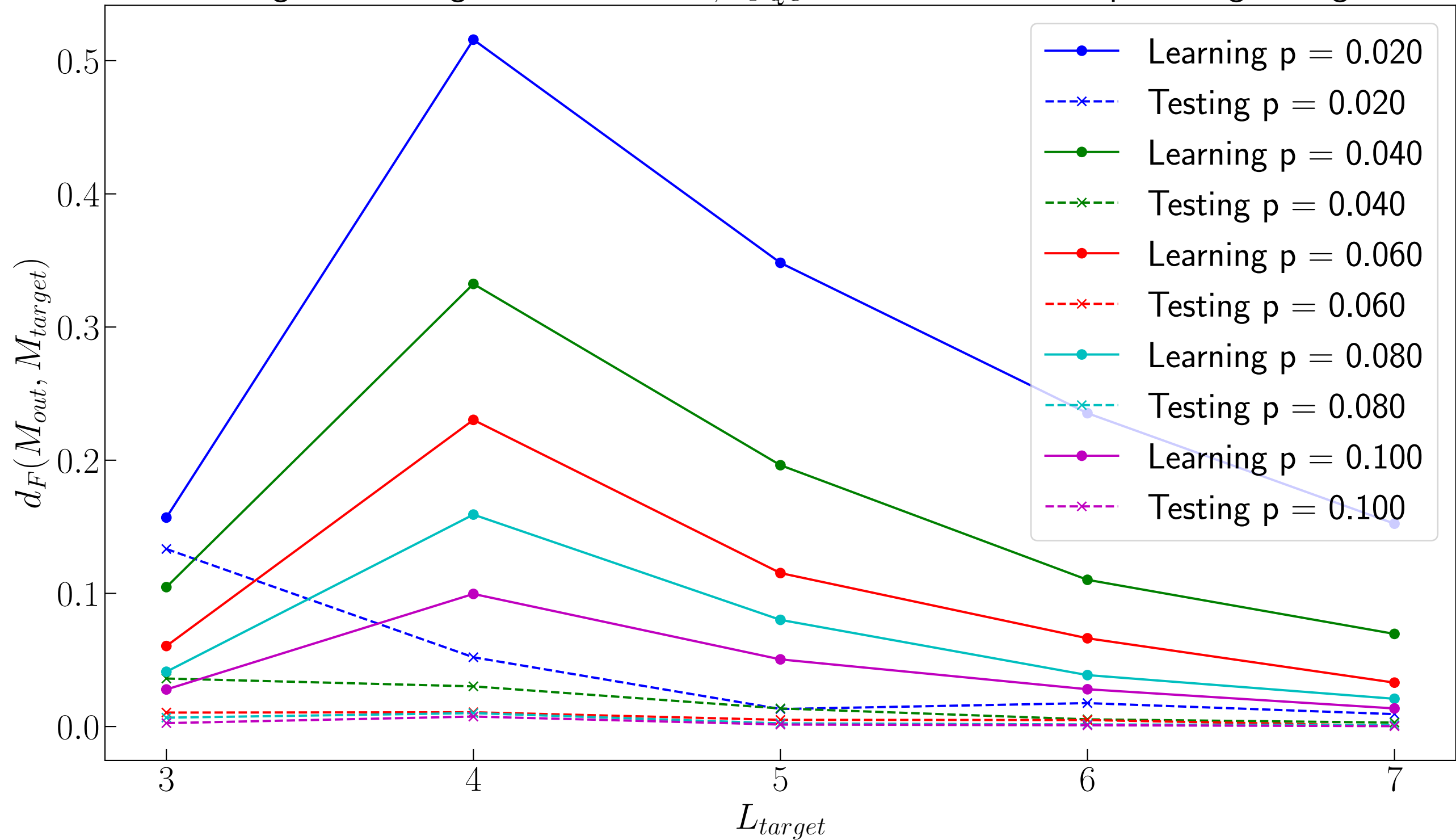
Learning and Testing Loss for N = 30, T_{PQC} = 3 with Various Depolarizing Strengths
