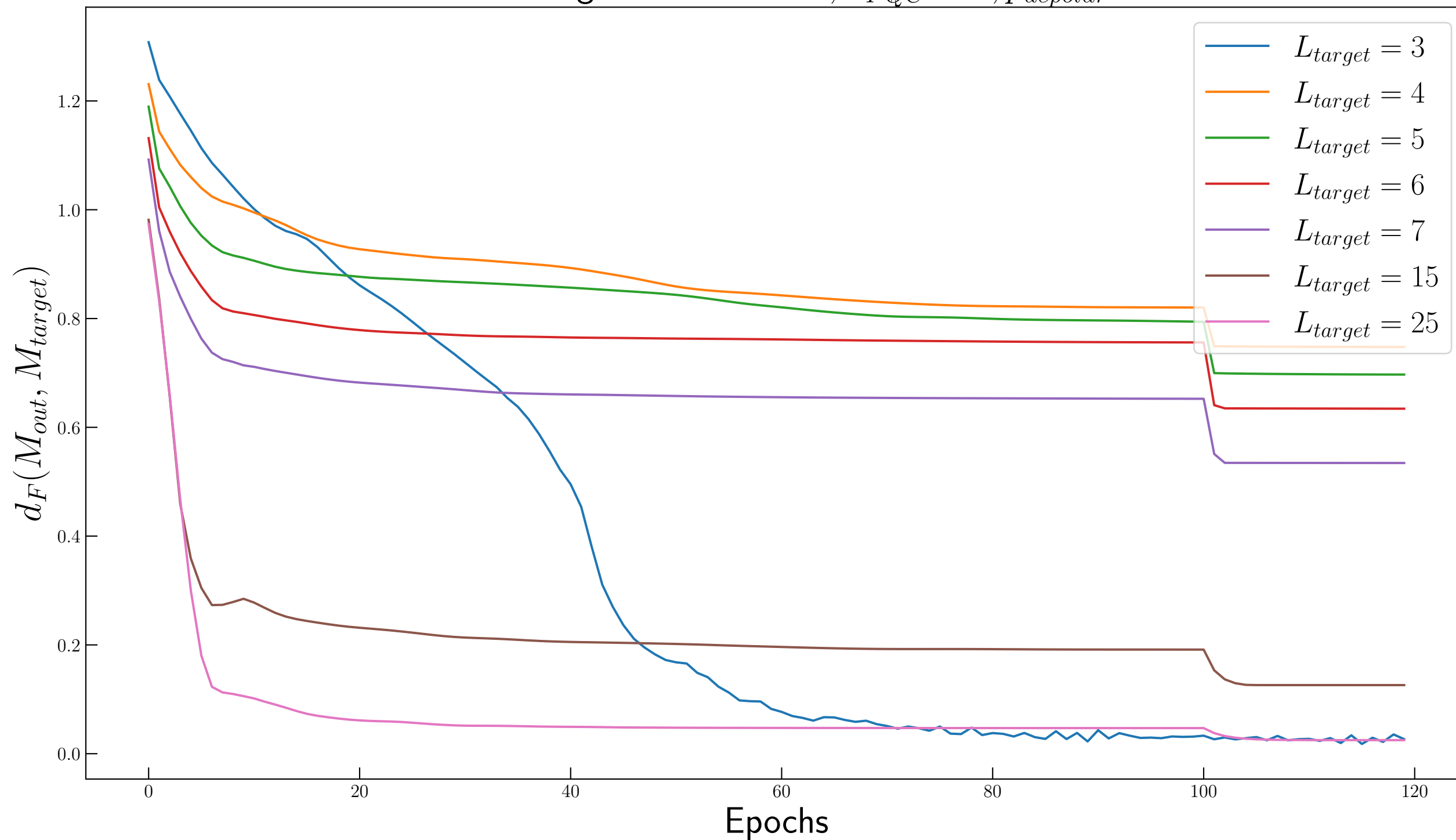
Trend of Learning Loss for N = 8, T_{PQC} = 2, p_{depolar} = 0.02
