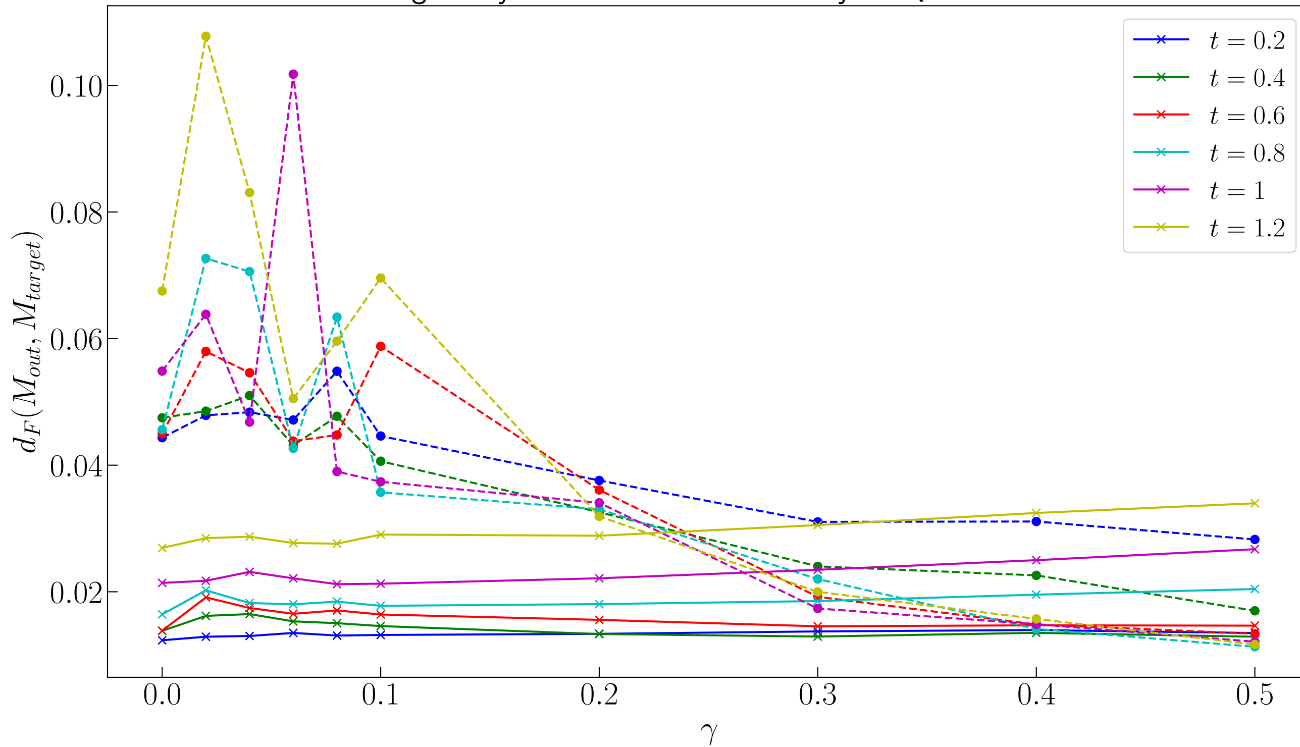
Learning 30-layer Trotterization with 3-layer PQC on 30 Sites
