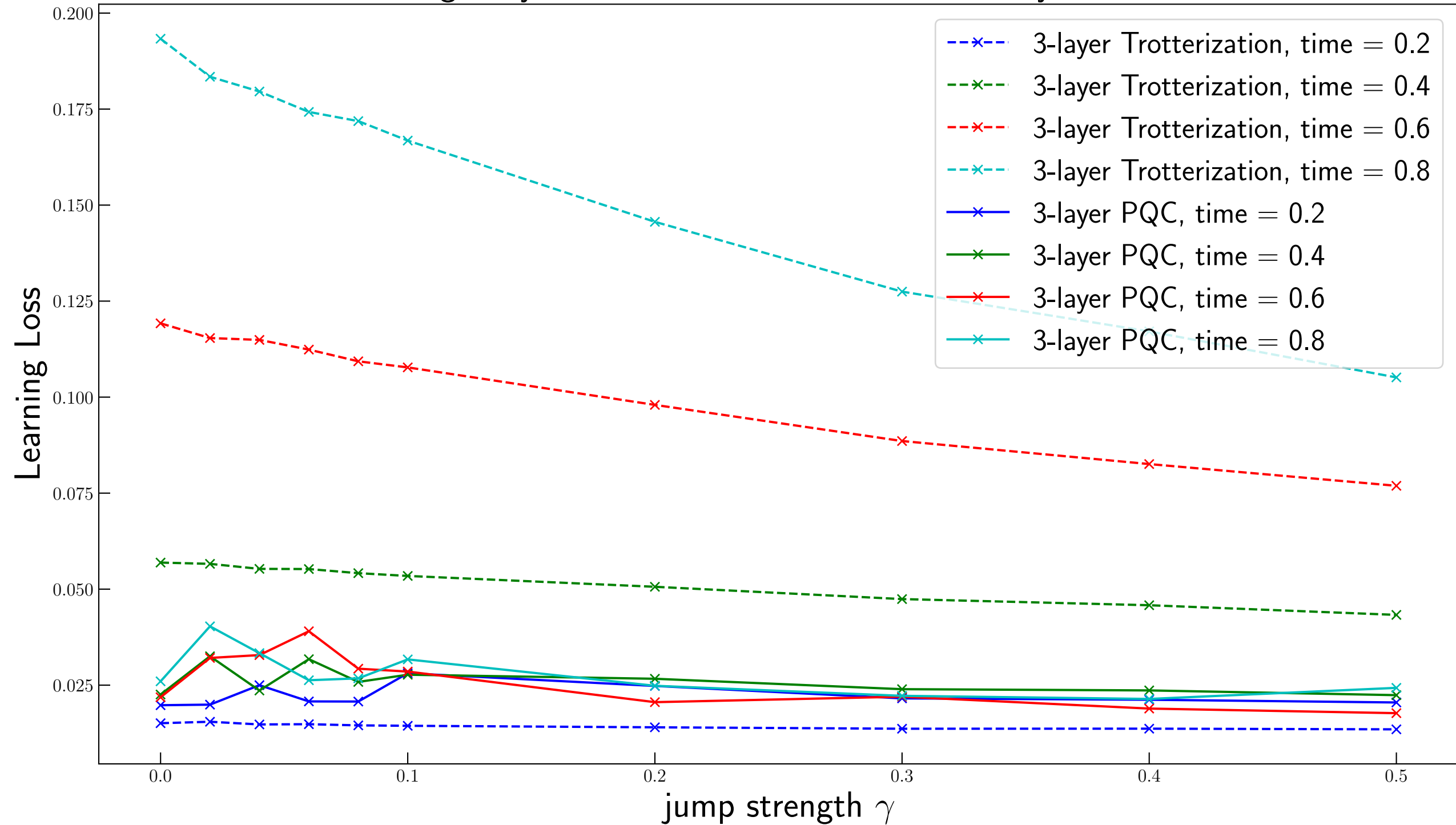
Loss of using 3-layer Trotterization or PQC to a 30-layer Trotterization
