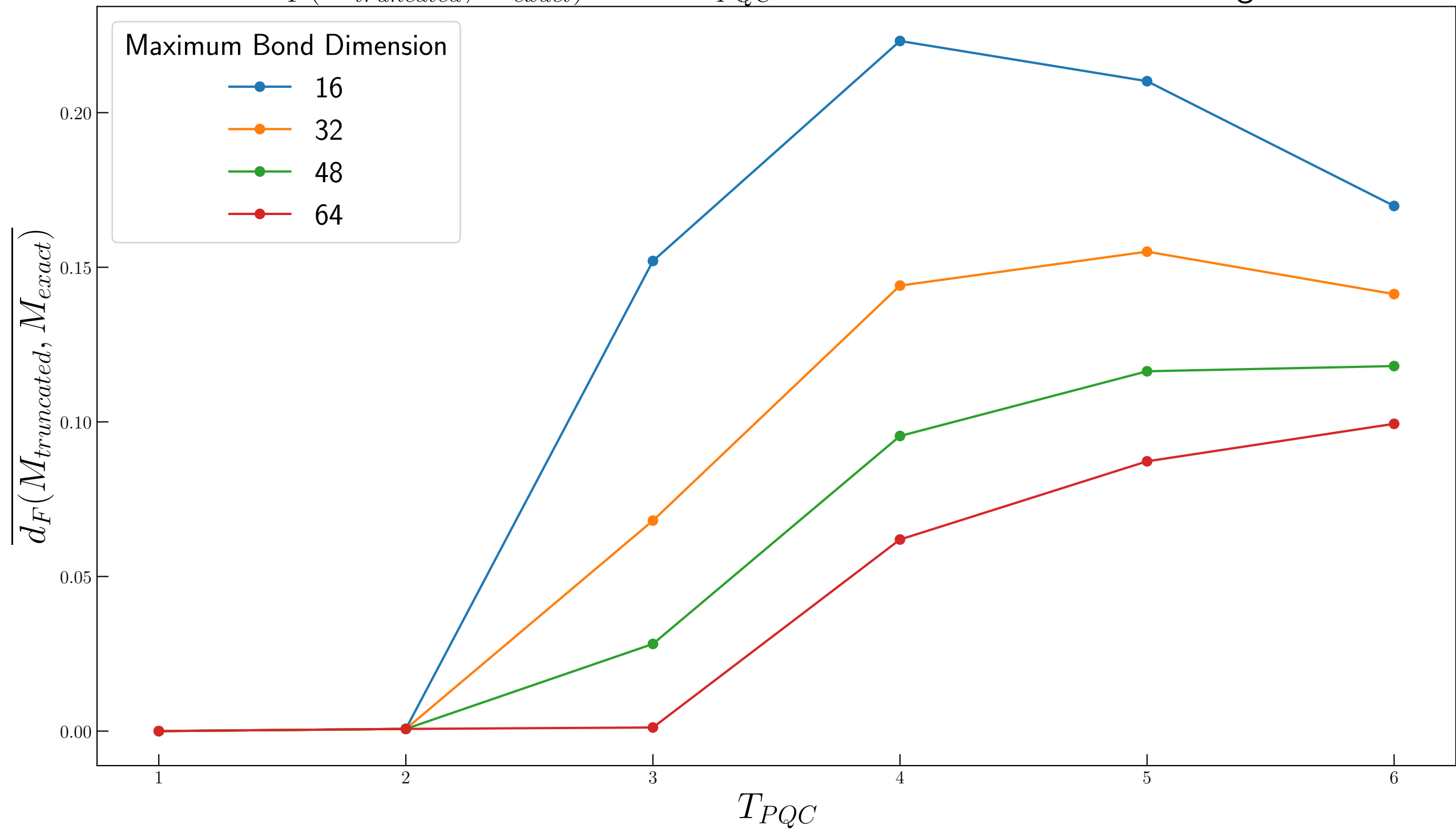
\overline{d_F(M_{truncated}, M_{exact})} versus T_{PQC} with Different Truncation Strength
