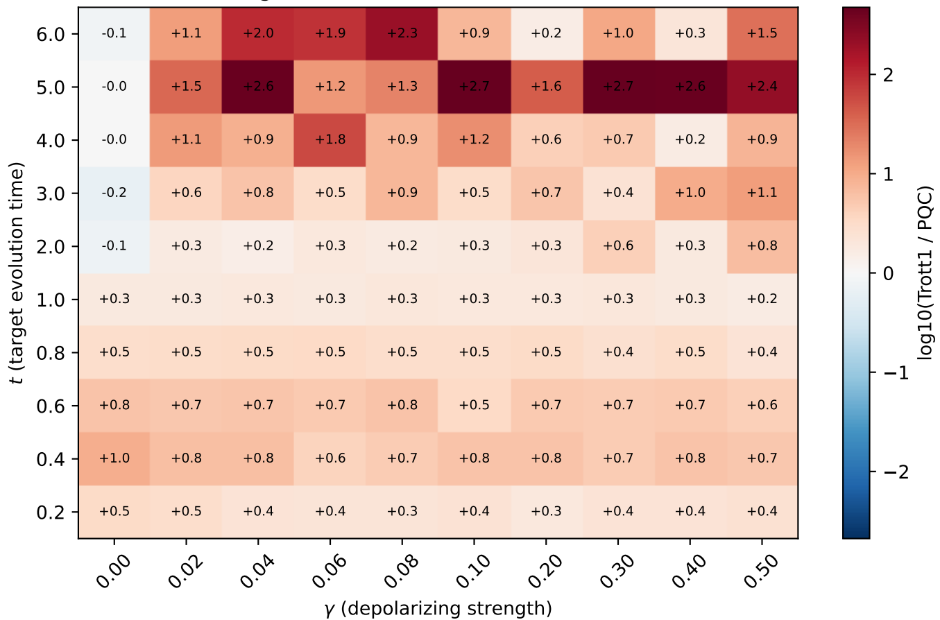
1st-order Trotter vs PQC \log_{10}(\text{Trott1} / \text{PQC}); + \rightarrow \text{PQC better}
