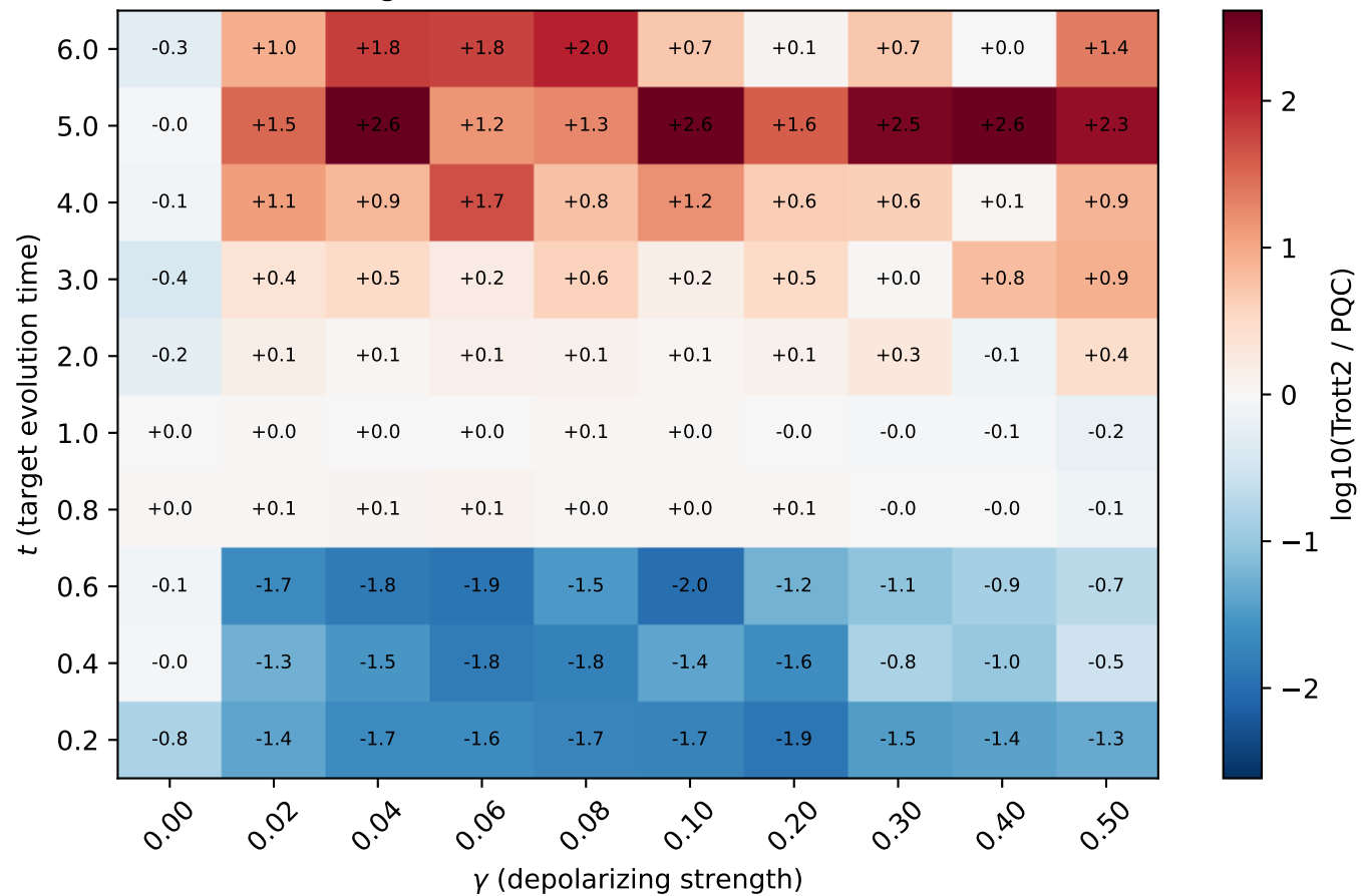
2nd-order Trotter vs PQC \log_{10}(\text{Trott2} / \text{PQC}); + \rightarrow \text{PQC better}
