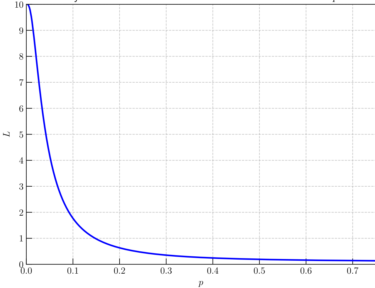
Layer L when the LOE reaches maximum as a function of p
