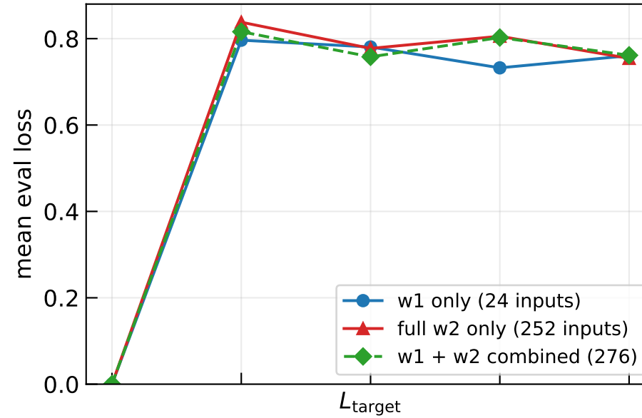
p = 0.01 , weight-2 eval
