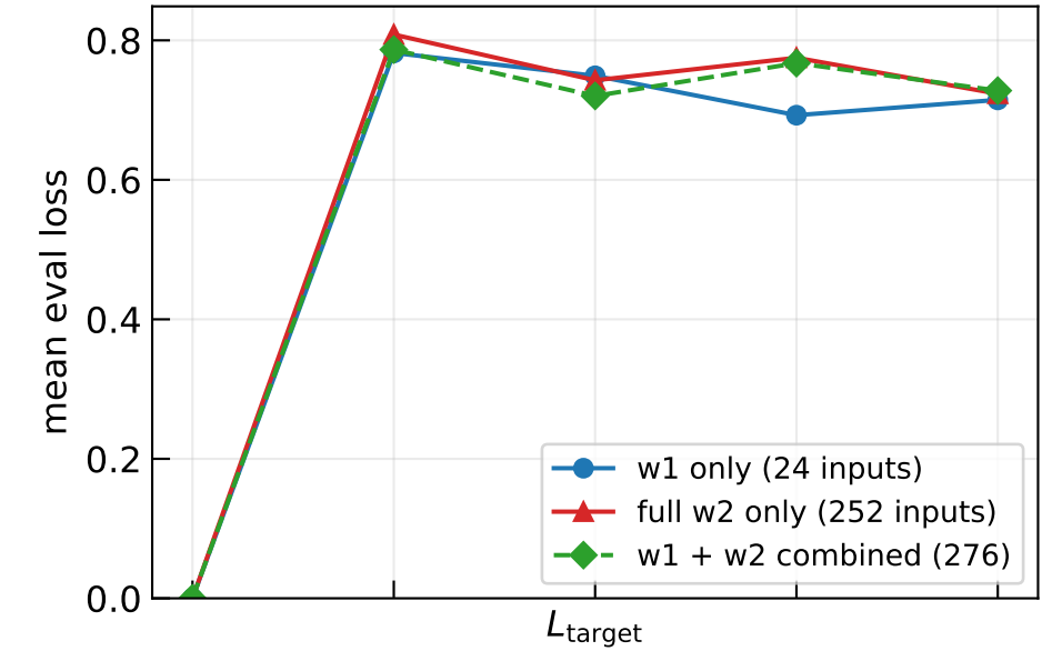
p = 0.01 , random Pauli eval
