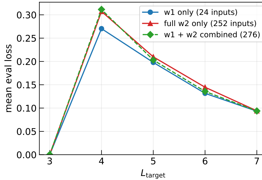
p = 0.05 , weight-2 eval
