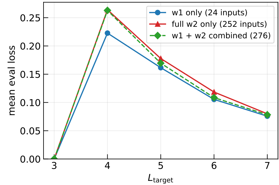
p = 0.05 , random Pauli eval
