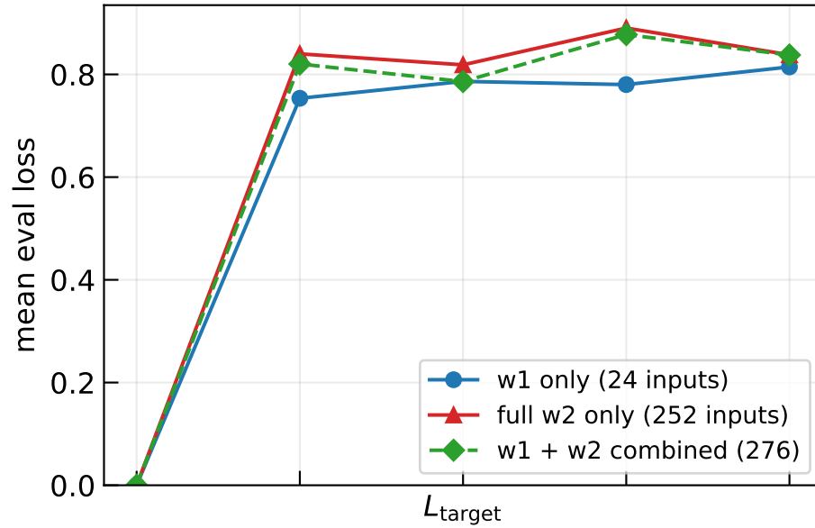
p = 0.01 , weight-1 eval
