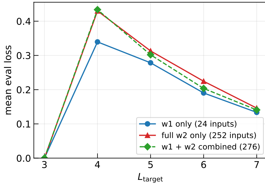
p = 0.05 , weight-1 eval
