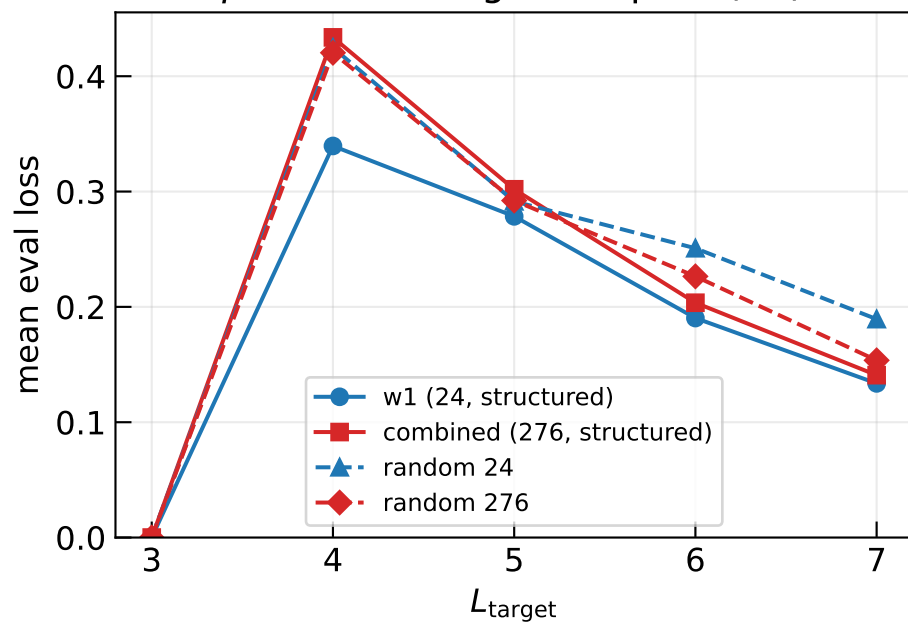
p = 0.05 , weight-1 inputs (24)
