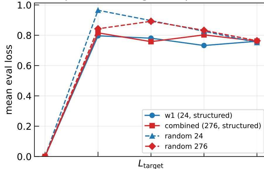
p = 0.01 , weight-2 inputs (84)
