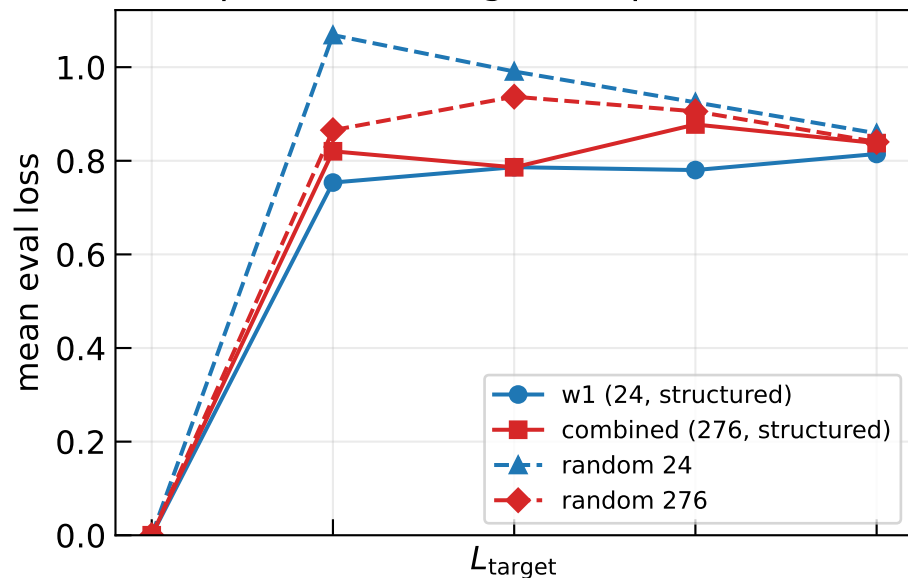
p = 0.01 , weight-1 inputs (24)
