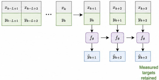
(a) Teacher forcing
