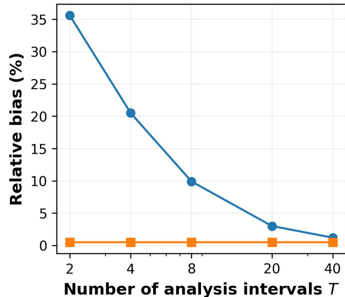
(a) Coefficient bias
