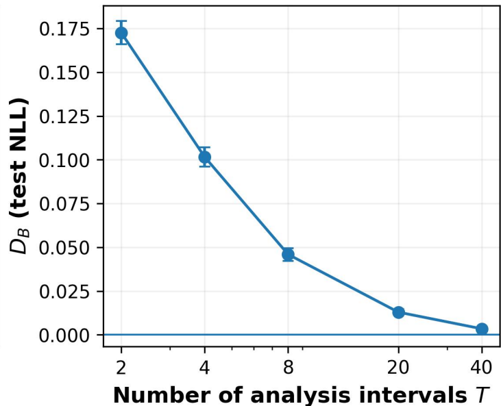
(b) Held-out likelihood difference
