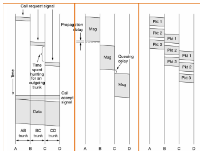
Figure 2.5: Confronto switching
