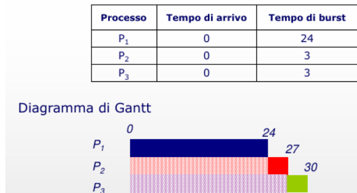
Figure 6.2: FCFS
