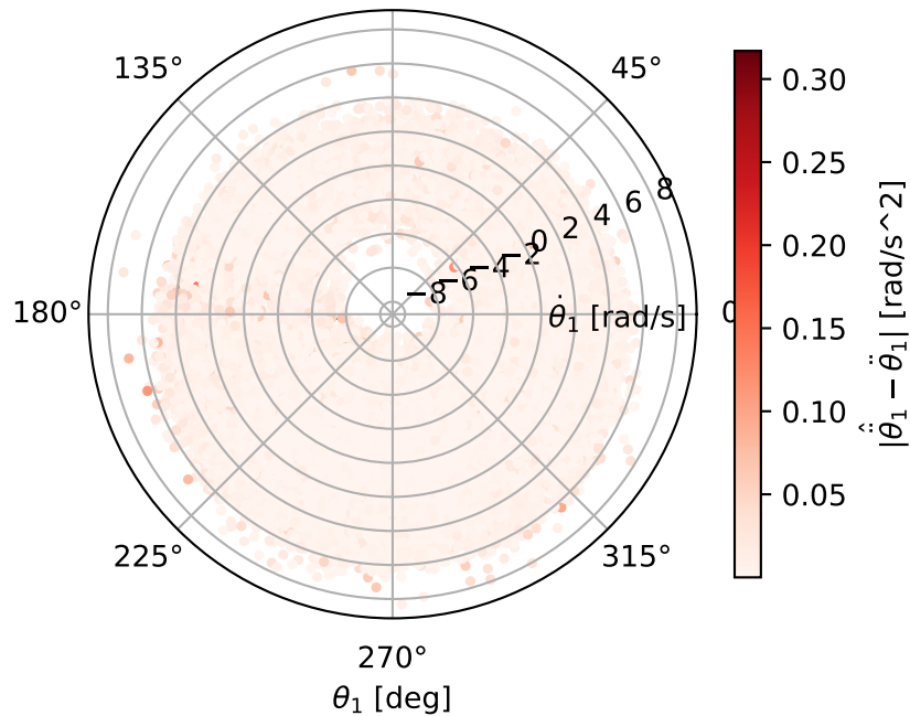
First link 90°
