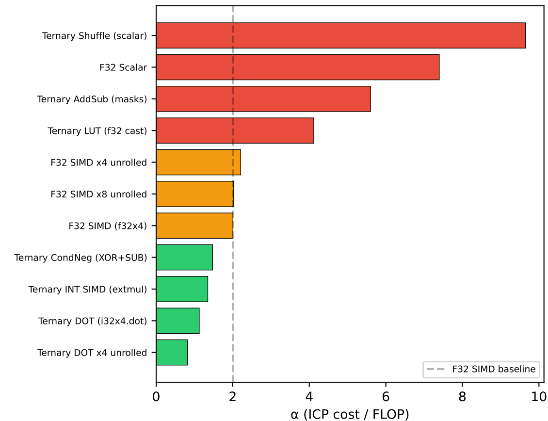
A. Kernel instruction cost
