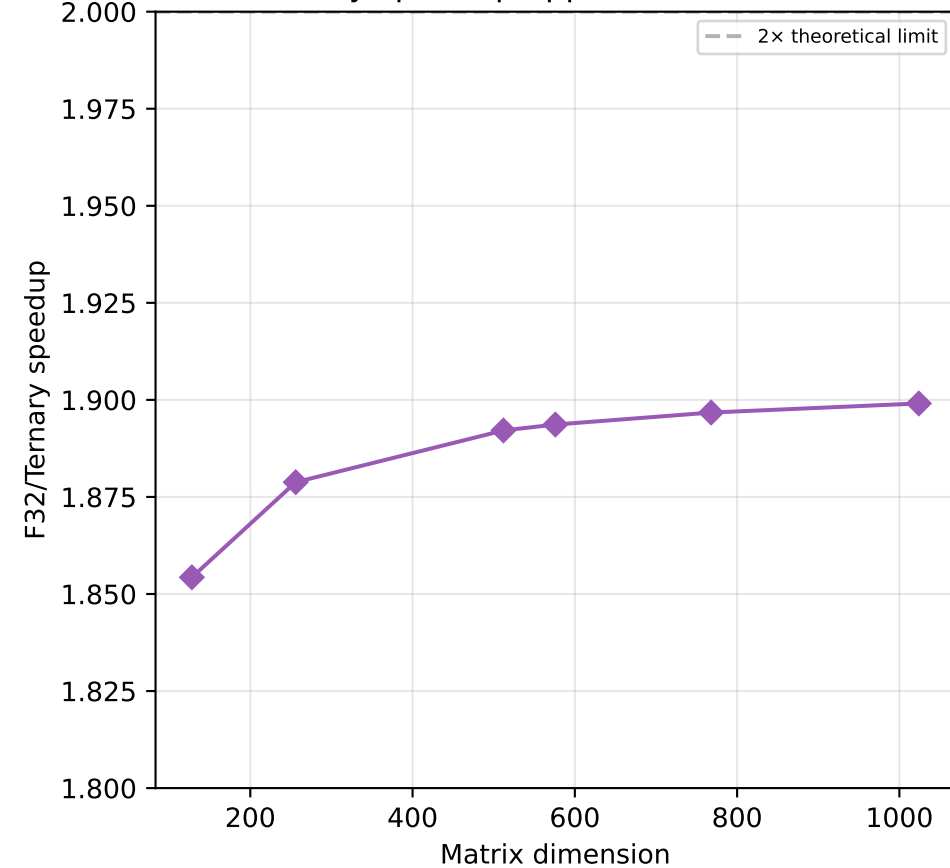
C. Ternary speedup approaches 2x at scale
