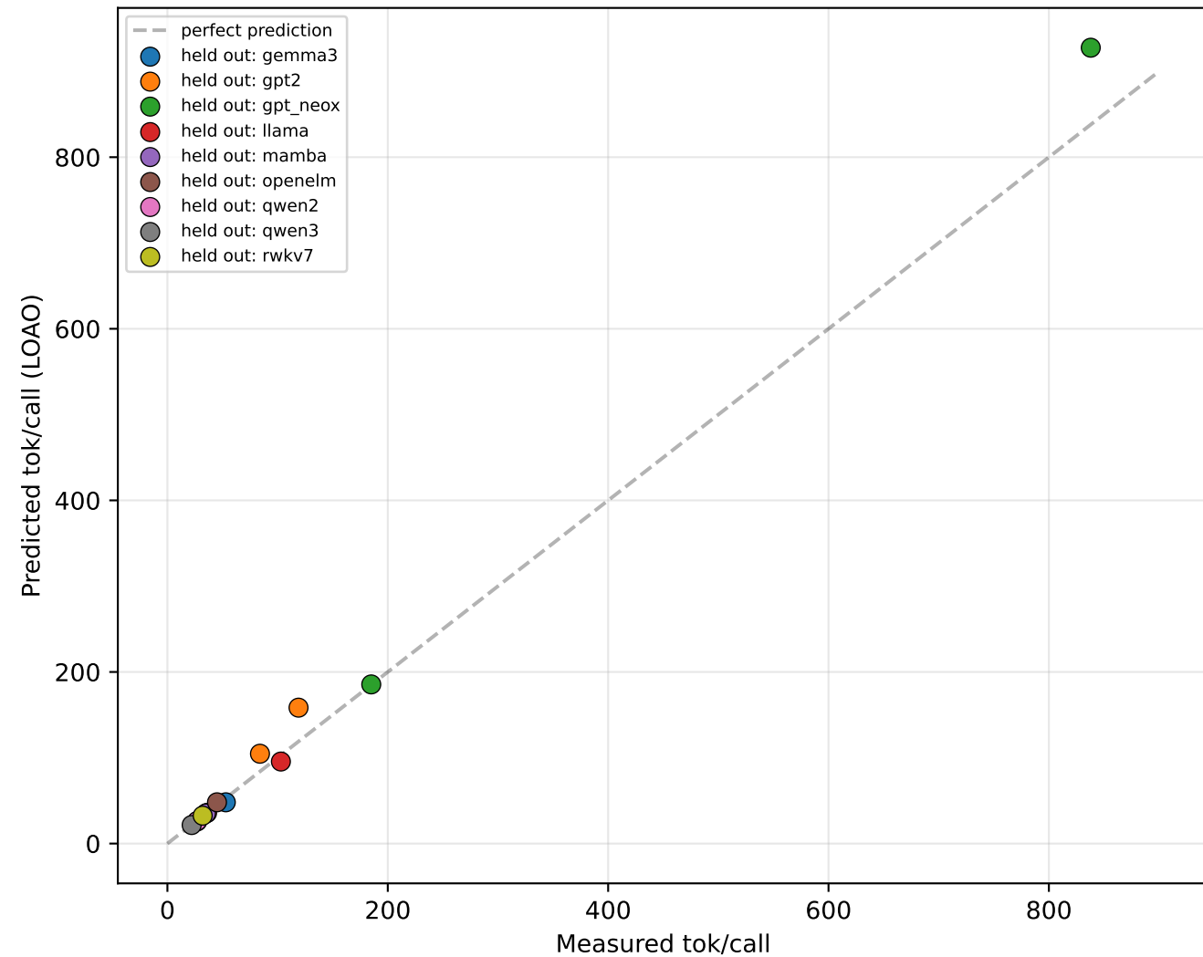
B. Leave-One-Architecture-Out validation
