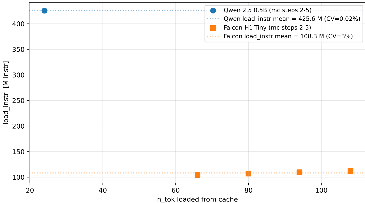
C3: re-attach (cache load) cost across multi-call steps 4× lower absolute cost for hybrid SSM vs Transformer
