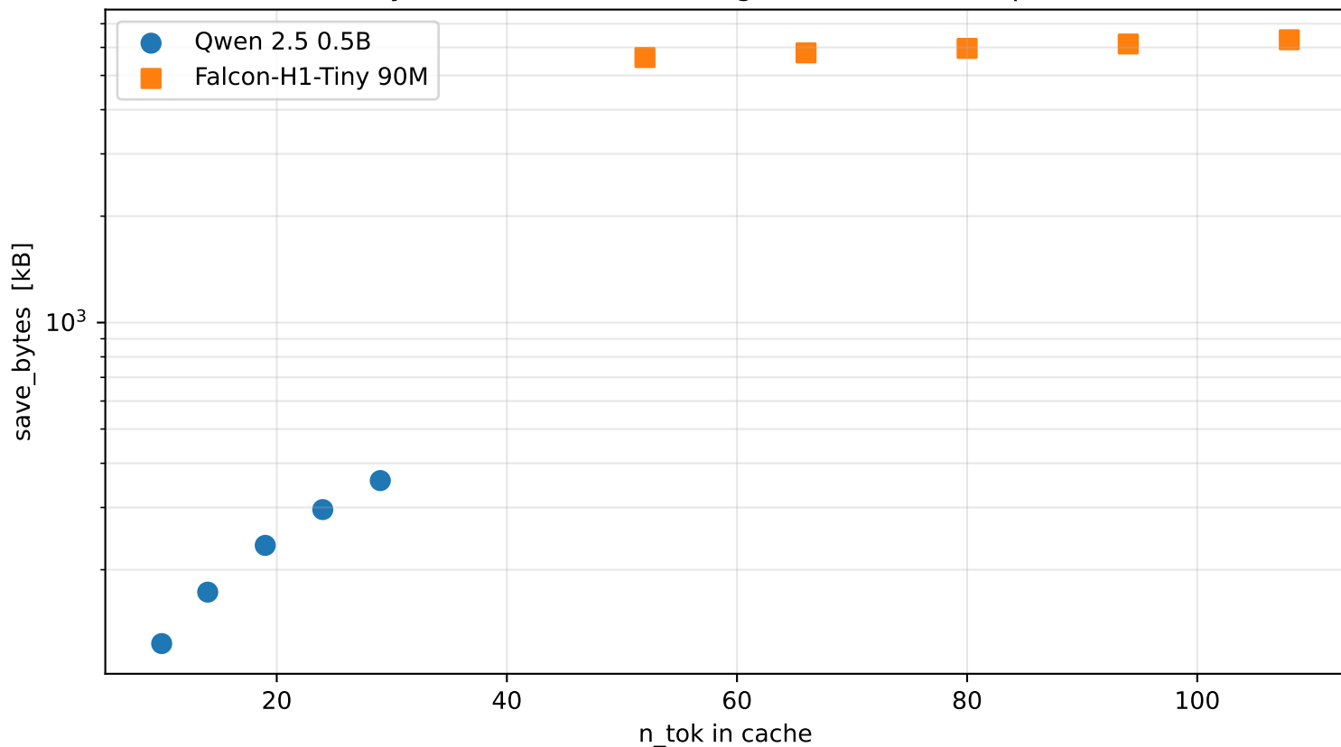
C3: serialized cache size (hybrid SSM has \sim 50\times larger fixed state footprint)
