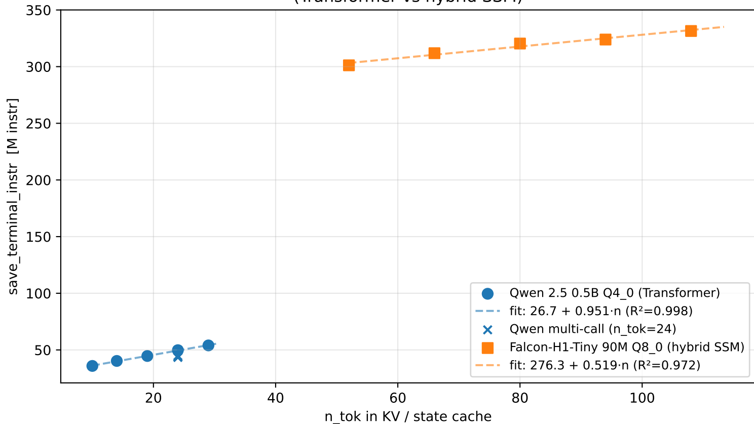
C3: per-call cache save cost scales with cache size (Transformer vs hybrid SSM)
