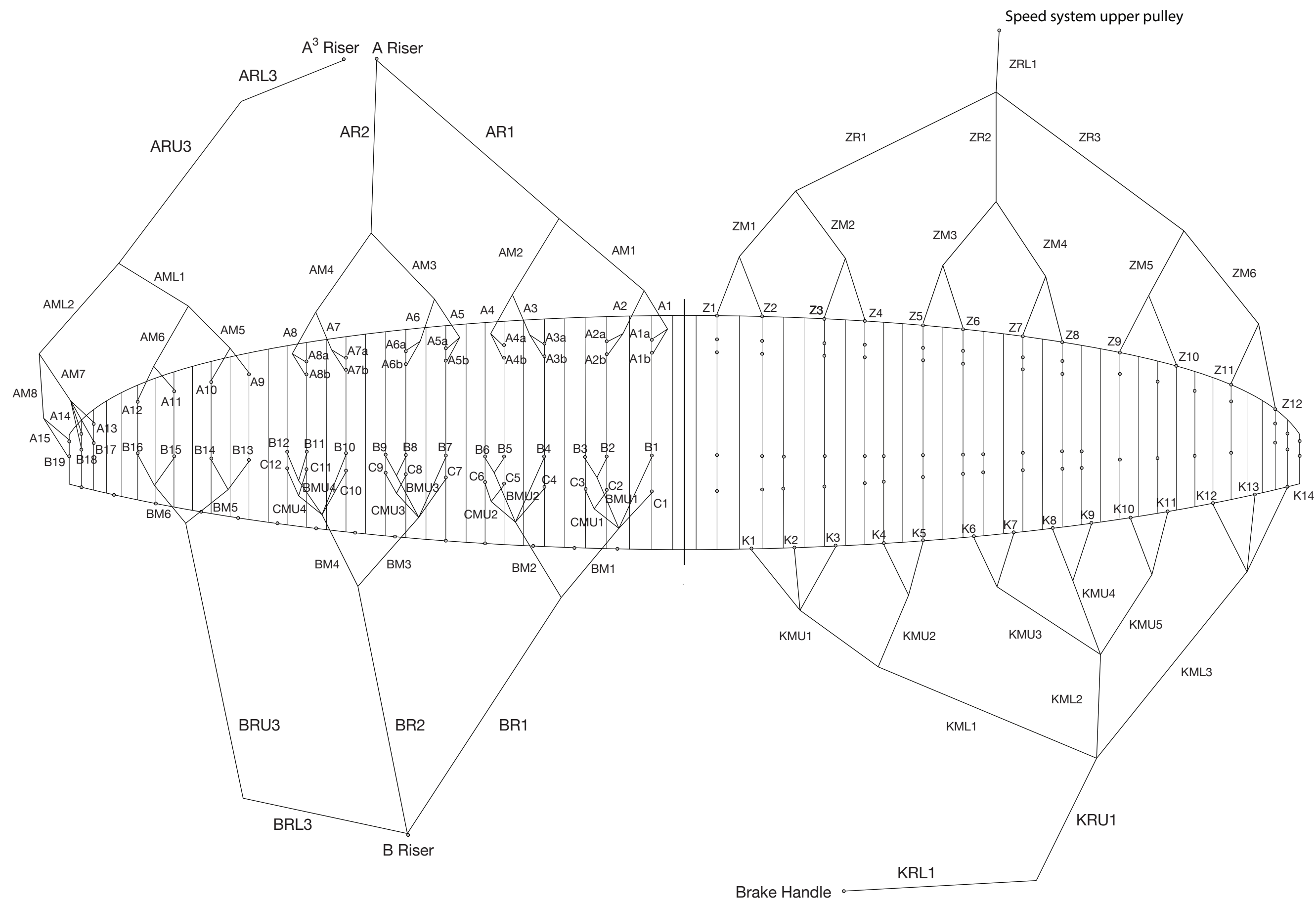
Alpina 5 Rigging Diagram
