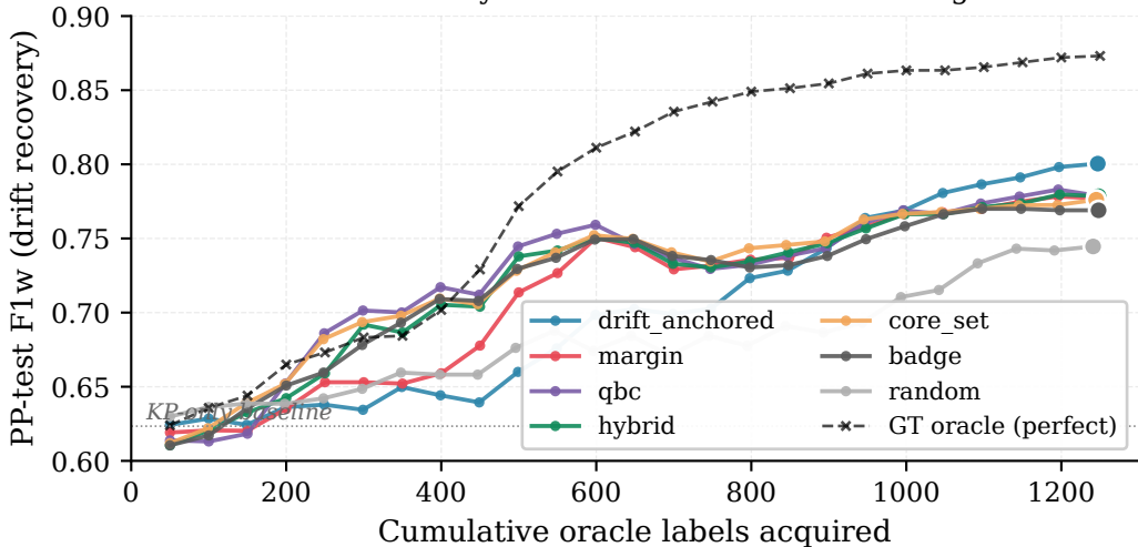
Label-efficiency Pareto across selection strategies
