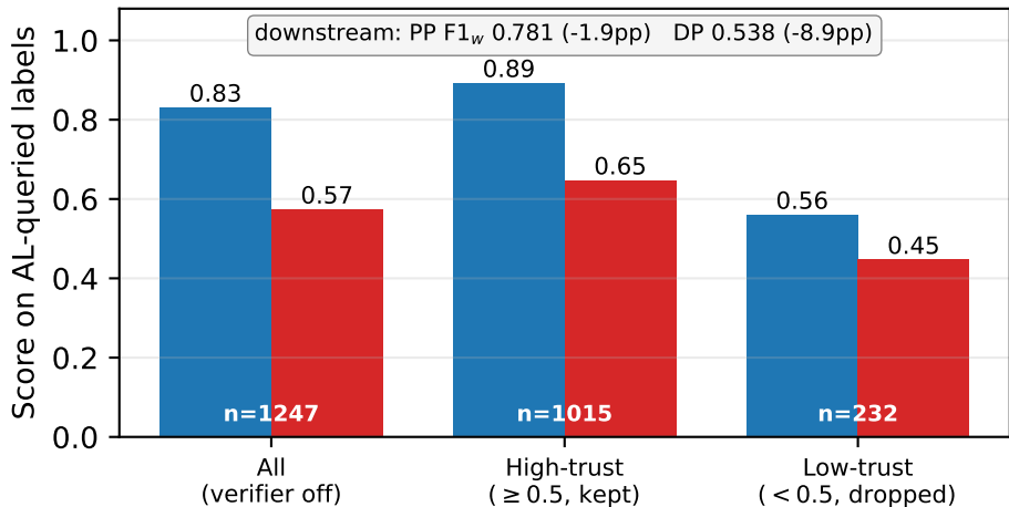
Oracle accuracy Oracle recall on phishing Verifier mode: T3 (OSINT coherence)
