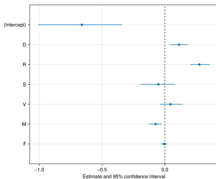
Fig. S3: Effect of anthelmintic intervention on vaccine responsiveness.
