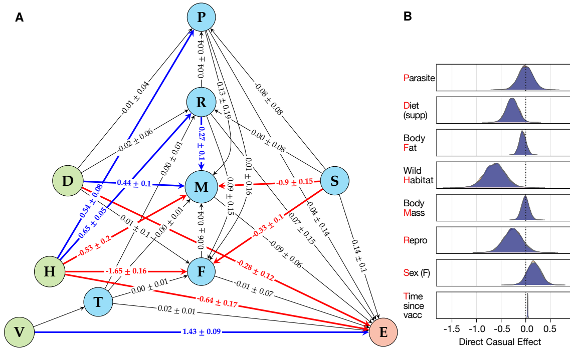
Fig. 4: Fully resolved Causal Model of vaccine efficacy. A. Directed acyclic graph representing point estimates of positive (blue) and negative (red) direct causal effects \pm std driving vaccine responsiveness E . B. MCMC sampling of posterior distributions of the coefficients for E := \beta_{DE}D + \beta_{FE}F + \beta_{HE}H + \beta_{ME}M + \beta_{PE}P + \beta_{RE}R + \beta_{SE}S + \beta_{TE}T (see Model parameterisation methods).
