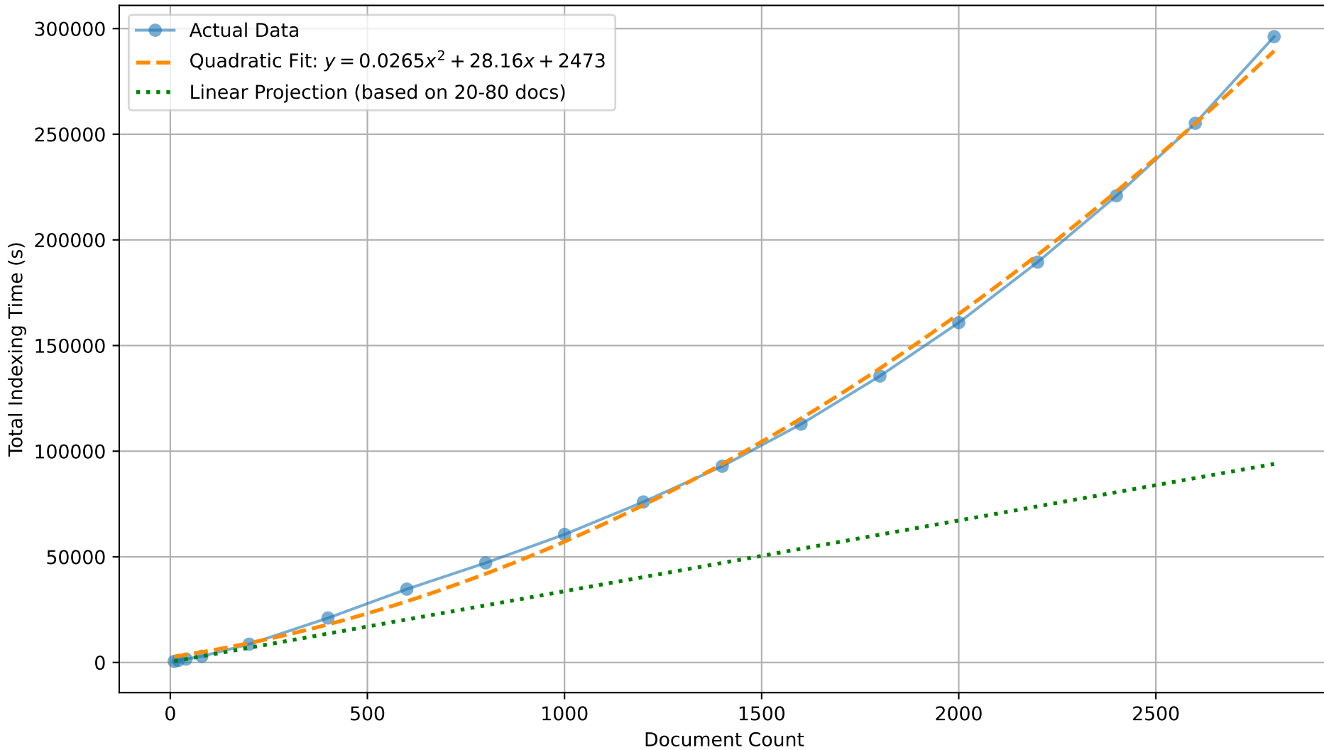
Total Indexing Time vs Document Count
