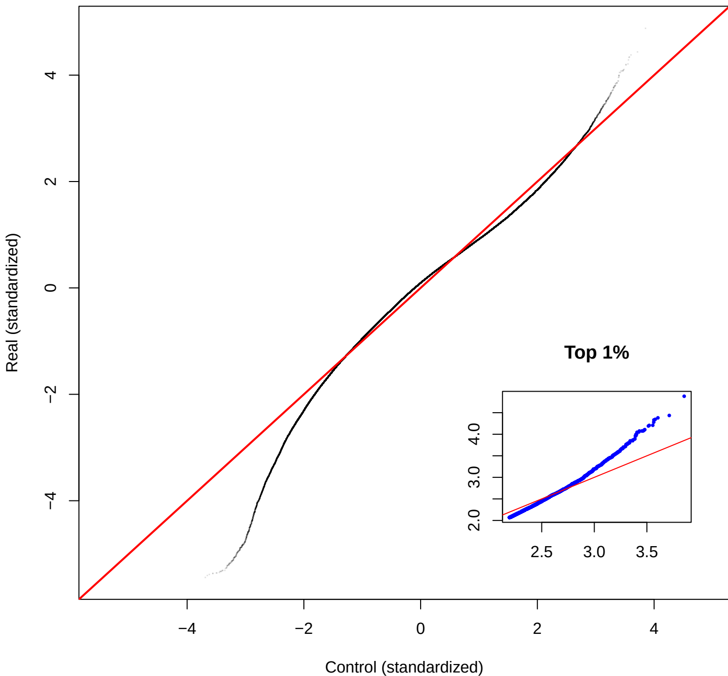
QQ Plot: Real vs Matched Normal Control
