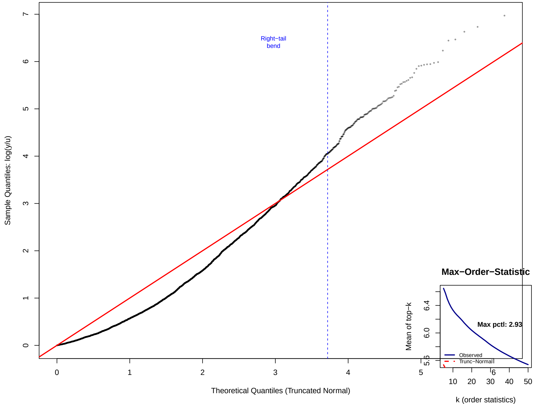
Tail Adequacy: Q-Q (2019, u=454.27, n=3165)
