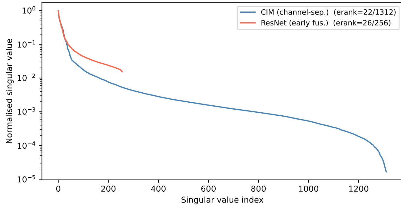
Singular value spectrum
