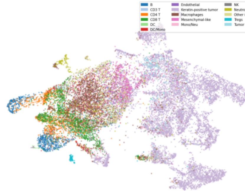
EarlyFusion32
