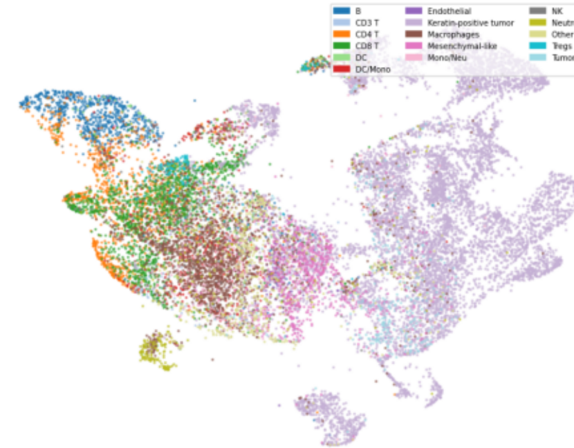
ResNet
