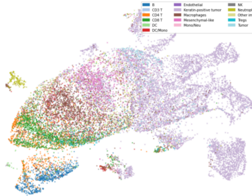
CIM_ProgFusion
