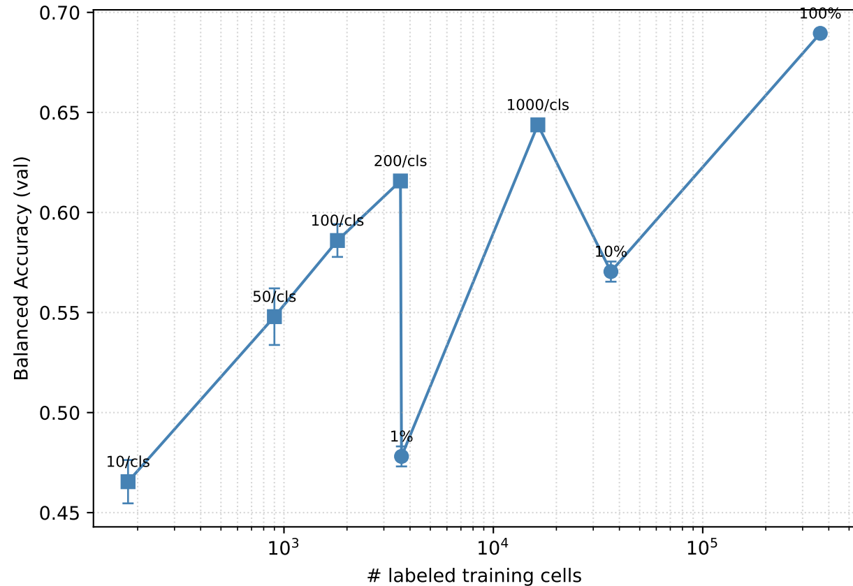
Label Efficiency — EarlyFusion32
